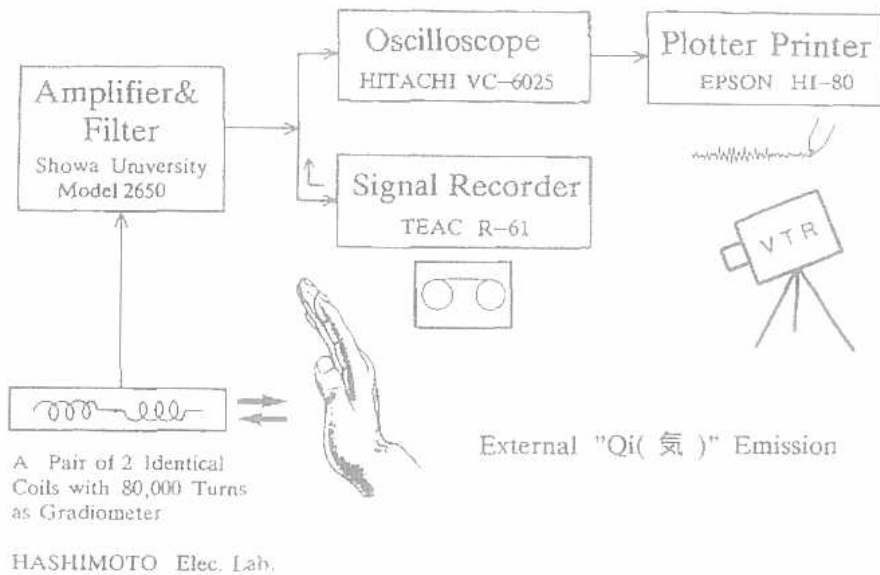
Fig. 6 : Composition of bio-magnetic field emission measurement system.
