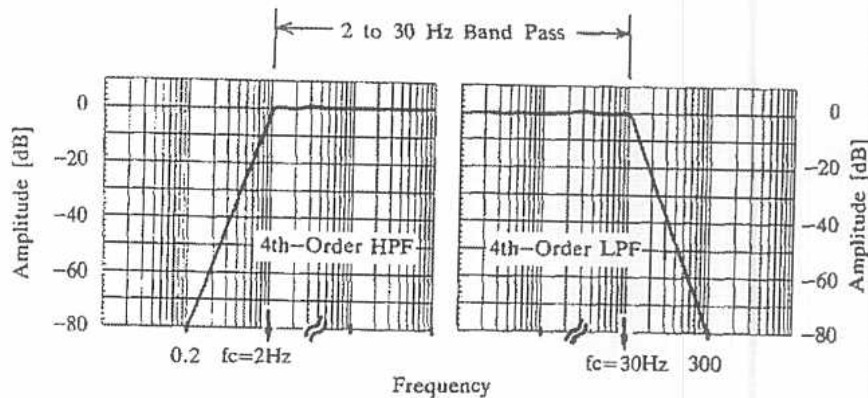
Fig. 5 : Sharp cutoff-frequency ( f_c ) characteristic of 4th-Order filter. Amplitude of the output-signal passed through the filter, is reduced in inverse proportion to " f^4 ", therefore called 4th-Order.
